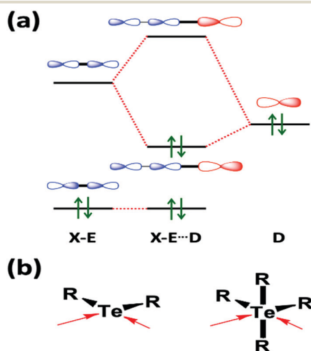
Fig. 7 (a) Simplified depiction of orbital interactions in secondary bonding and (b) the preferred directions of the secondary bonds around tellurium(II) and tellurium(IV).
