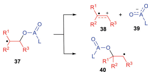
Scheme 9 Heterolytic dissociations and 1,2-shifts of \beta -(acyloxy)alkyl and \beta -(phosphatoxy)alkyl radicals.
