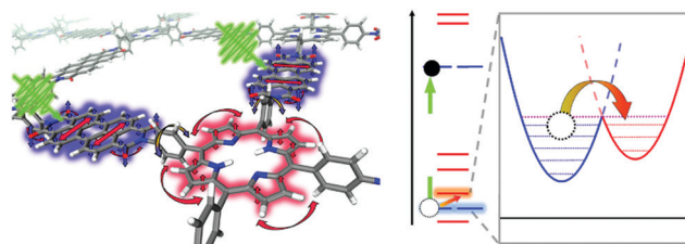
Fig. 17 Schematic overview of phonon-assisted charge carrier dynamics in the photo-excited PDI-porphyrin COF. The rotation of the phenyl ring correlates with the \pi -interactions between the PDI and the porphyrin linkers, leading to ultrafast hole transfer from PDI to the porphyrin macrocycle. Reproduced with permission. 70 Copyright 2019, Nature Publishing Group.
