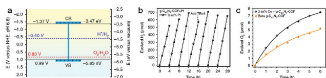
Fig. 24 (a) Bandgap diagram with marked potential for HER and OER. (b) Hydrogen and (c) oxygen production during photocatalytic water splitting based on g-C 40 N 3 -COF. Reproduced with permission. 27 Copyright 2019, Nature Publishing Group.
