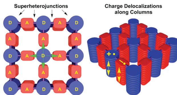
Fig. 13 Illustration of segregated donor-acceptor columns in D_{MPC}-A_{DI} -COF. Photoinduced electron transfer occurs directly to the adjacent acceptor and also to diagonally disposed acceptors. Charge carrier migration is depicted as arrows along the columns. Reproduced with permission. 69 Copyright 2015, American Chemical Society.
