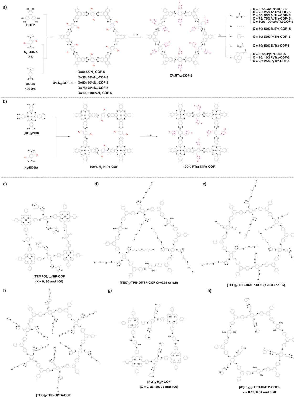
Fig. 31 Pore surface engineering of (a) X\%N_3\text{-COF-5} and (b) 100\% N_3\text{-NiPc-COF} . (c–h) Representative examples of post-synthetic modified COFs from azide–alkyne click reaction.
