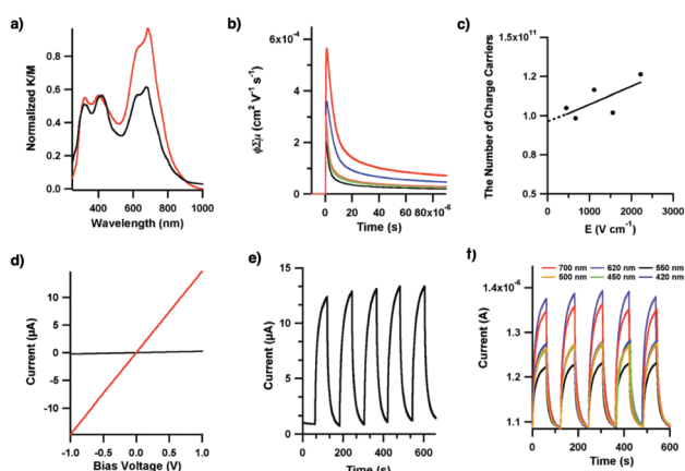
Fig. 41 (a) Electronic absorption spectra of 2D-NiPc-BTDA COF (red curve) and [\text{MeO}]_8\text{PcNi} (black curve). (b) Transient conductivities when irradiated with a 355 nm pulsed laser at a photon density of 1.6 \times 10^{15} under Ar (red curve) and \text{SF}_6 (blue curve) and after annealing under \text{SF}_6 for 1 h (orange curve) and 24 h (green curve) or under \text{O}_2 for 24 h (black curve). (c) Numbers of charge carriers measured by the time-off light transient current integration at different bias voltages, when irradiated with a 355 nm pulsed laser of 5.0 \times 10^{14} photons \text{cm}^{-2} . (d) I - V curves of 2D-NiPc-BTDA COF in the dark (black curve) and upon irradiation (red curve) with visible light. (e) On-off switching of the photocurrent of 2D-NiPc-BTDA COF at a bias voltage of 1.0 V, by switching the light on and off. (f) Wavelength-dependent on-off switching of photocurrent at a bias voltage of 1.0 V. Adapted with permission from ref. 386, Copyright 2011 ACS.
