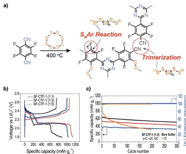
Fig. 73 (a) Synthetic scheme for the synthesis of SF-CTF-1s involving elemental sulphur-mediated nitrile trimerisation along with the simultaneous covalent attachment of elemental sulphur via S n Ar chemistry. (b) The first discharge-charge curves of SF-CTF-1s measured at 0.05C in the voltage range of 1.8–2.7 V. (c) Cycling performance and coulombic efficiencies of SF-CTF-1 (1:3) at 1C, 2C and 5C over 300 cycles (1C = 1000 mA g -1 ). Adapted with permission from ref. 437, Copyright 2017 Wiley-VCH.
