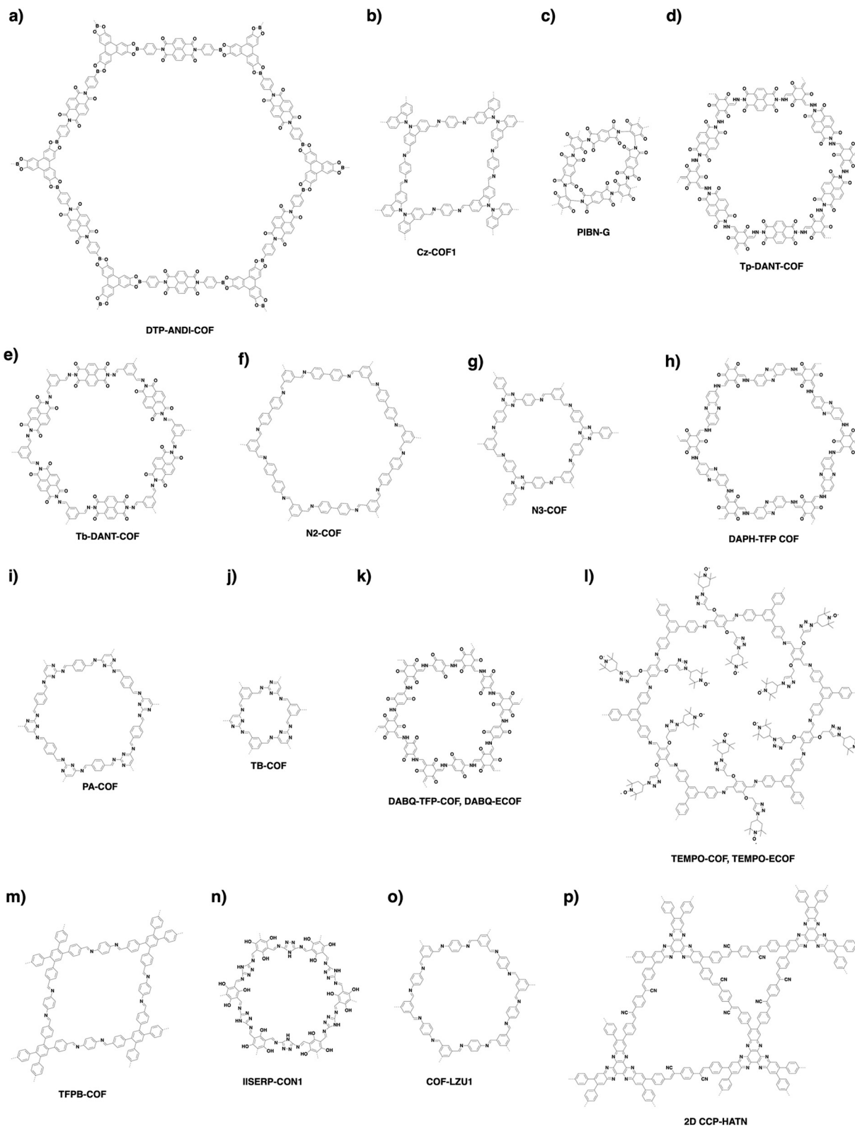
Fig. 77 Structures of COFs designed as electrodes for lithium ion batteries.
