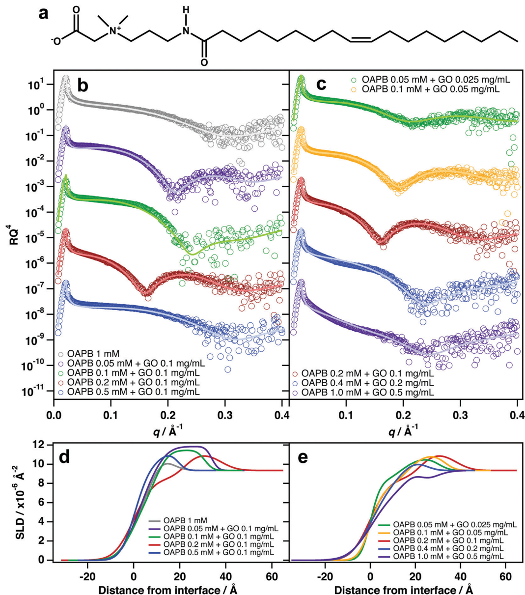
Fig. 4 (a) Chemical structure of oleyl amidopropyl betaine (OAPB). (b) and (c) Air–water XRR datasets of different mixtures of OAPB and GO at (b) different ratios and at (c) a fixed ratio but different loadings. Vertical error bars have been removed and the data have been vertically offset for clarity. (d) and (e) SLD profiles generated from the model fits shown in (b) and (c) respectively.
