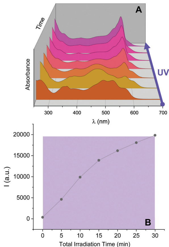
Fig. 4 Evolution of the absorbance (top panel) and integrated emission intensity (bottom panel, \lambda_{\text{ex}} = 550 nm) of a solution of 2NB-RZ (18 \mu\text{M} , 20 °C, \text{CH}_3\text{OH} , \text{NH}_2\text{OH} 3000 eq.) before and after irradiation at 365 nm (0–30 min, 5 min irradiation intervals).
