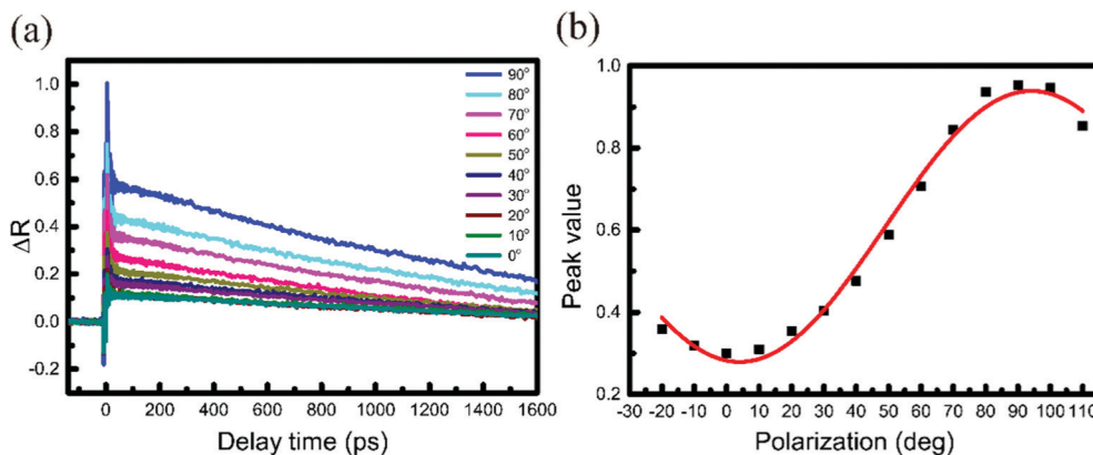
Fig. 4 (a) TR traces, recorded for a series of beam polarizations ranging from 0^\circ to 90^\circ , where the pump and probe polarization directions were parallel to each other. The beam polarization angle is shown in Fig. 1(b). The pump (520 nm) and probe (1040 nm) beam fluences were 8 and 4.8 \mu\text{J cm}^{-2} , respectively. (b) Peak differential reflection signal as a function of beam polarization angles with respect to sample orientation.
