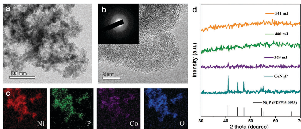
Fig. 11 Laser fragmentation in water to synthesize amorphous multi-component metal oxide NPs. (a) TEM and (b) HRTEM images of amorphous CoNiPO 4 NPs; (c) corresponding elemental mapping including Ni, P, Co and O; (d) the XRD patterns of CoNi 2 P particles before fragmentation and laser-fragmented CoNiPO 4 NPs under different pulsed energies: 369, 480 and 541 mJ. Reproduced with permission from ref. 203.
