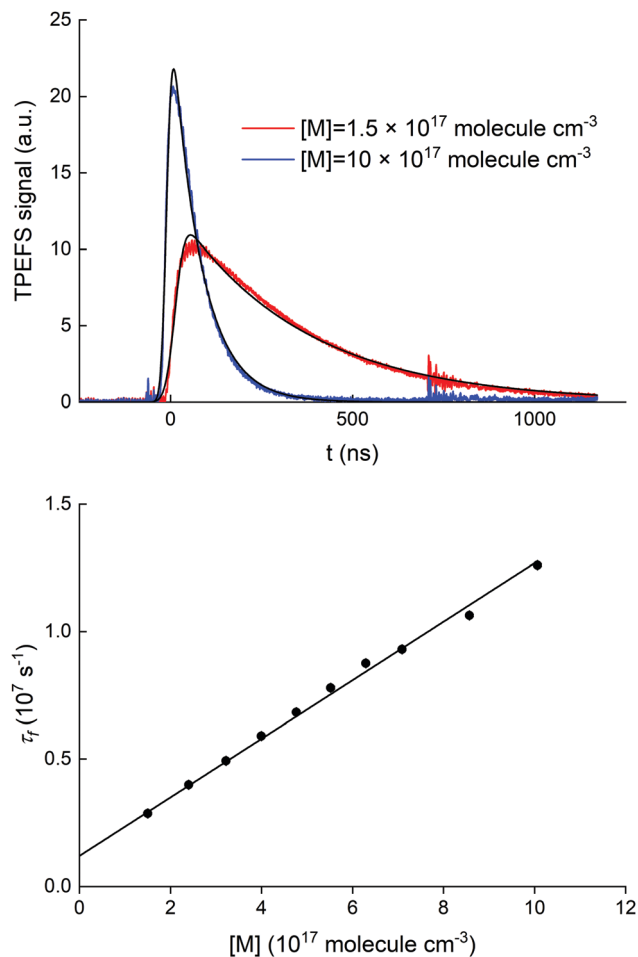
Fig. 4 Upper panel: Time resolved fluorescence signal detected by the PMT through the (310 ± 5) nm interference filter following the 193 nm excitation of HNO 3 . The black, solid lines correspond to fits using (E2). Lower panel: Fluorescence decay constant ( \tau_f ) versus bath gas (N 2 ) concentration. The black solid line corresponds to a linear regression used for fitting \tau_f . Error bars are 2 \sigma statistical only.
