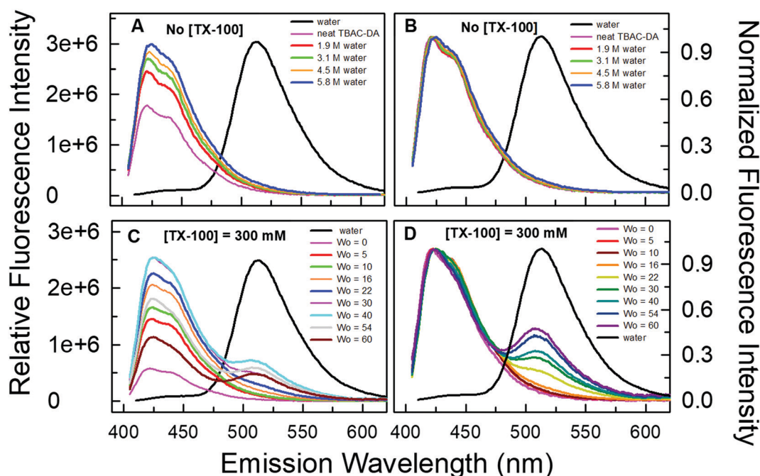
Fig. 4 Relative (panels A and C) and normalized (panels B and D) fluorescence emission spectra of pyranine (10 μM, \lambda_{ex} = 390 nm, and slits: excitation/emission = 2/2 nm) dissolved within neat DES TBAC-DA and TX-100(300 mM)/TBAC-DA systems at different amounts of water loading ( w_0 ), respectively. The fluorescence emission spectrum of pyranine in water is also included in each panel for reference.
