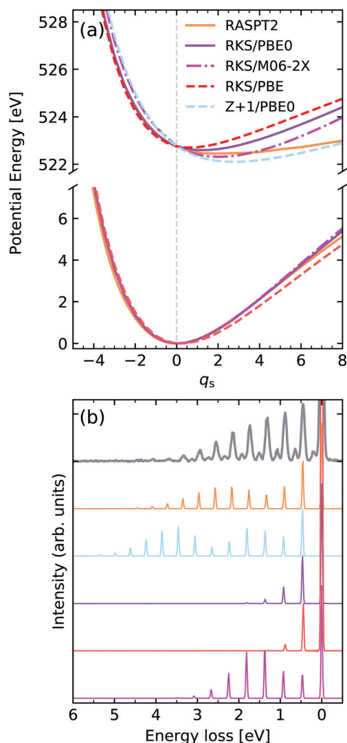
Fig. 10 (a) Potential energy curves along the dimensionless symmetric stretching coordinate of water for the ground state (bottom) and |\text{O } 1s^{-1}2b_2\rangle core-excited state computed employing different functionals and methods. For comparability, the vertical transition point of all curves were matched to the one of the RKS/PBE0 PEC. The vertical transition point is marked by a dashed gray line. (b) Experimental vibrational RIXS spectrum of water 2 along with the theoretical spectra computed with the respective potential curves displayed in panel (a).
