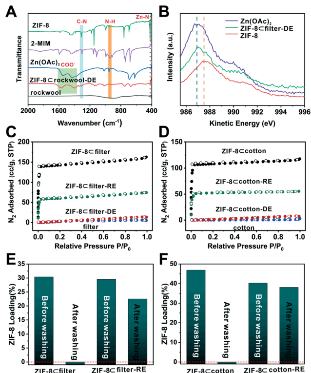
Fig. 4 (A) The FTIR spectrum of ZIF-8, 2-MIM, \text{Zn}(\text{OAc})_2 , ZIF-8 \subset rockwool-DE and rockwool. (B) The Zn LMM Auger spectrum of \text{Zn}(\text{OAc})_2 , ZIF-8 and ZIF-8 \subset filter-DE; 77 K \text{N}_2 sorption isotherms of (C) ZIF-8 \subset filter and (D) ZIF-8 \subset cotton during the degradation–reconstruction cycle; ZIF-8 loading of (E) ZIF-8 \subset filter and ZIF-8 \subset filter-RE before and after washing and (F) ZIF-8 \subset cotton and ZIF-8 \subset cotton-RE before and after washing.
