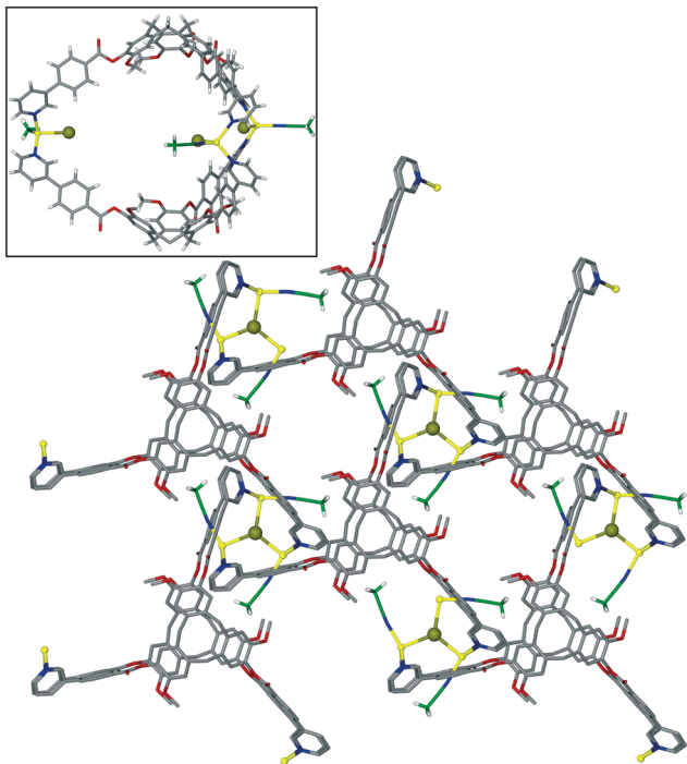
Fig. 7 From the structure of [\text{Ag}_3(\text{L10})_2(\text{CH}_3\text{CN})_3\text{Cl}] \cdot 2\text{AsF}_6 \cdot n(\text{CH}_3\text{CN}) showing the 2D network of \text{Ag}_3\text{L}_2 capsules linked by \mu_3\text{-Cl}^- (larger olive spheres) and inset is side-view of one capsule highlighting that the \mu_3\text{-Cl}^- are endo to the cage. 13
