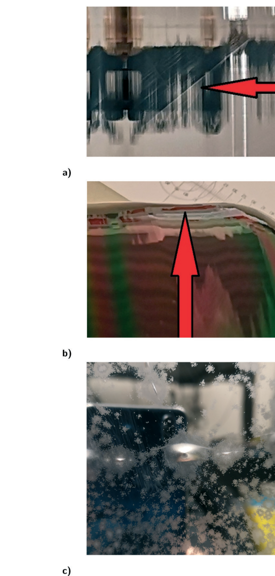
Fig. 8 Sample anomalies. a) Slip lines on sample 1, b) diameter anomalies on sample 2 near start of shoulder cone, c) close up image of sample 2 end-face near its apex showing surface defects and solidified droplets.
