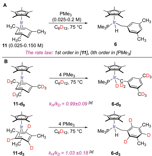
Fig. 4 (A) The model reaction to determine reaction order in Cp*Ir ( \eta^4 -mesitylene) ( 11 ) and \text{PMe}_3 . (B) Thermolysis of 11-d 9 and 11-d 3 ; kinetic isotope effects and the lack of H/D scrambling. [a] KIEs were calculated from the initial rates for separate reactions of the deuterated and non-deuterated species.
