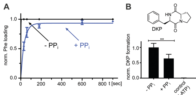
Fig. 6 Effect of excess \text{PP}_i on the aminoacylation reaction of full-length wt NRPS modules. (A) Time-course of L-Phe-Pant thioester formation of full-length holo-GrsA monitored by ESI-MS. GrsA (10 \mu\text{M} ) was mixed with ATP/L-Phe (each 2 mM) and \text{PP}_i (5 mM) as indicated. Shown are fitted curves of normalized data with the mean \pm SD of three independent experiments ( k_{\text{with PP}_i} = (2.9 \pm 0.2) \times 10^{-2} \text{ s}^{-1} ). (B) Dipeptide product formation by full-length modules holo-GrsA and holo-TycB1. GrsA (0.5 \mu\text{M} ) was mixed with TycB1 (5 \mu\text{M} ), ATP (5 mM), L-Pro and L-Phe (each 2 mM), and \text{PP}_i (5 mM) as indicated. The formed D-Phe-L-Pro-diketopiperazine (DKP) was analyzed and quantified by HPLC. Shown are the mean \pm SD of three independent replications. ** indicates p \leq 0.01 , which was determined by Student's t -test.
