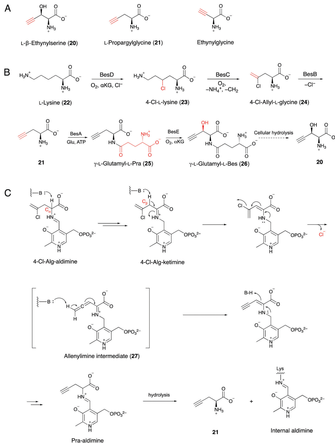
Fig. 8 (A) Terminal-alkyne amino acids from Streptomyces spp. (B) Proposed biosynthetic pathway of βes from L-lysine. (C) Putative mechanism for BesB-catalyzed formation of Pra ( 21 ) from 4-Cl-allylglycine ( 24 ).
