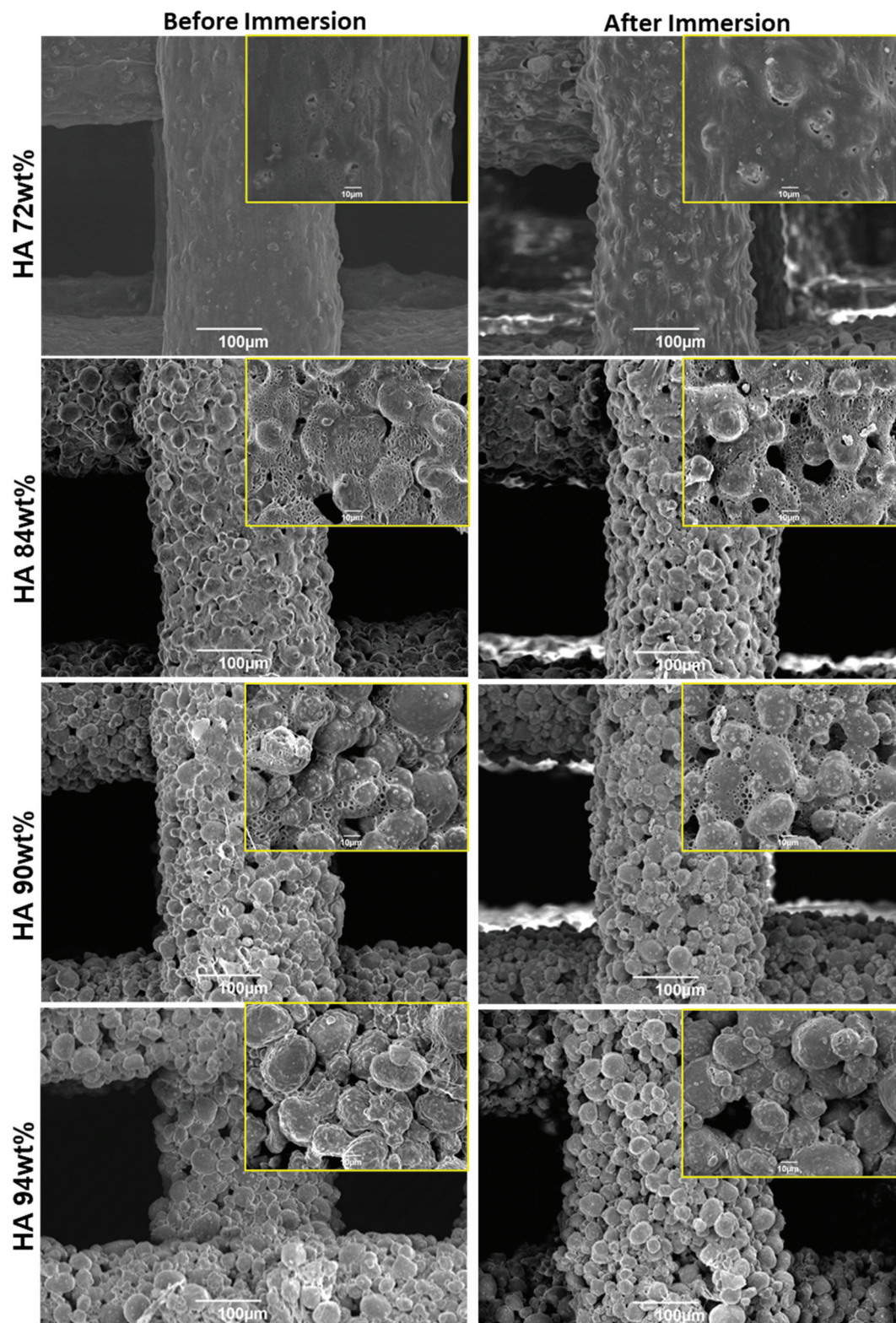
Fig. 7 SEM images of PCL/PEG(400)/HA scaffolds with varied HA concentrations. Insets show the high-magnification images of strut surfaces. The scale bars in insets are 10 \mu\text{m} .
