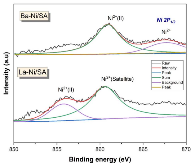
Fig. 6 Ni 2p XPS spectra of calcined X–Ni/SA catalysts.
