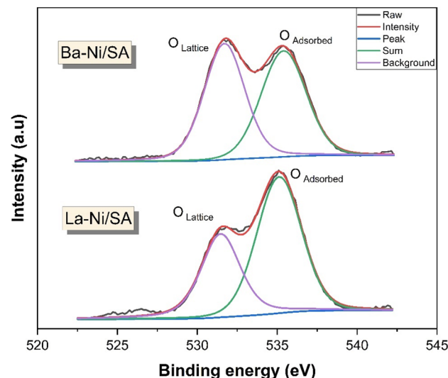
Fig. 7 O 1s XPS spectra of calcined X–Ni/SA catalysts.
