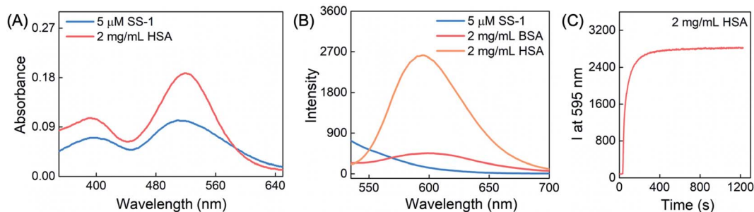
Fig. 1 Optical responses of SS-1 toward HSA. (A) UV-vis absorption changes upon addition of 2 mg mL -1 HSA into a 5 \mu M SS-1 -containing PBS system. (B) The corresponding changes in the fluorescence spectra. (C) Time-dependent fluorescence intensity change in the reaction system at 595 nm. \lambda_{\text{ex}} = 505 nm; \lambda_{\text{em}} = 525–700 nm; slit 5/5 nm; 700 V.
