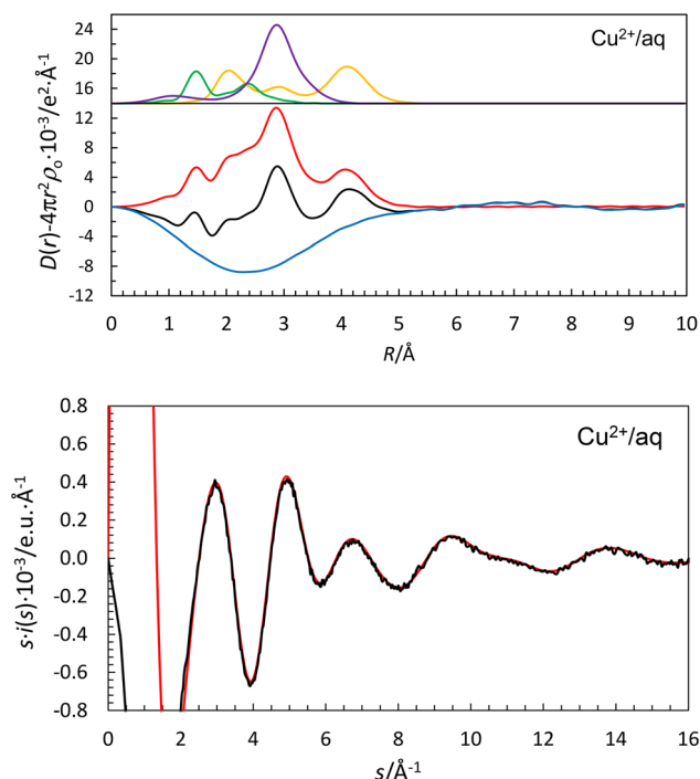
Fig. 5 (Top) LAXS radial distribution curves for a 1.50 mol dm -3 aqueous perchloric acidic solution of copper(II) perchlorate. Upper part: Separate model contributions (offset: 15) of the hydrated copper(II) ion (yellow line), the hydrated perchlorate ion (green line) and aqueous bulk (purple line). (Middle) Experimental RDF: D(r) - 4\pi r^2 \rho_0 (black line); sum of model contributions (red line); difference (blue line). (Bottom) Reduced LAXS intensity functions s \cdot i(s) (black line); model s \cdot i_{\text{calc}}(s) (red line).
