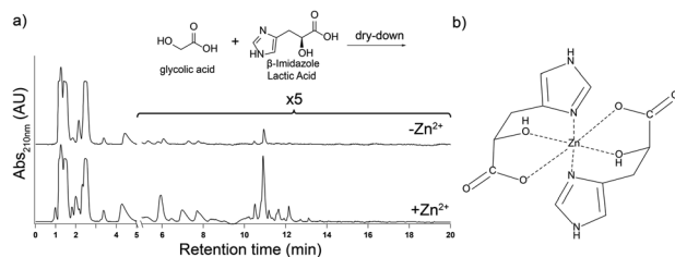
Fig. 4 Zinc increases lengths of his-containing polyesters in dry-down reactions. (a) L- \beta -Imidazole lactic acid (His) was dried with glycolic acid (glc) at a 1 : 1 molar ratio at 85 °C for seven days in the presence or absence of \text{Zn}^{2+} , at a 1 : 1 molar ratio of his to \text{Zn}^{2+} . Analysis of samples via C18-HPLC showed a dramatic increase in the yield of longer oligomers in the presence of \text{Zn}^{2+} . (b) Possible coordination complex between \text{Zn}^{2+} and his monomers.
