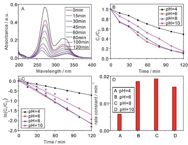
Fig. 5 (A) Time-course UV-vis absorbance spectra of CIP ( 10^{-5} M) photocatalyzed by 1 \text{ g L}^{-1} NaYF 4 :Yb,Tm@TiO 2 under Xe lamp at pH = 8. (B–D) The calculated time-dependent ratios of C_t/C_0 , first-order degradation rates and reaction rate constants for CIP ( 10^{-5} M) photocatalyzed 1 \text{ g L}^{-1} NaYF 4 :Yb,Tm@TiO 2 with different pH values.
