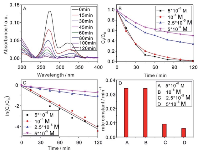
Fig. 4 (A) Time-course UV-vis absorbance spectra of CIP ( 10^{-5} M) photocatalyzed by 1 \text{ g L}^{-1} NaYF 4 :Yb,Tm@TiO 2 under Xe lamp. (B–D) The calculated time-dependent ratios of C_t/C_0 , first-order degradation rates, and reaction rate constants for different concentration of CIP photocatalyzed by 1 \text{ g L}^{-1} NaYF 4 :Yb,Tm@TiO 2 under Xe lamp.
