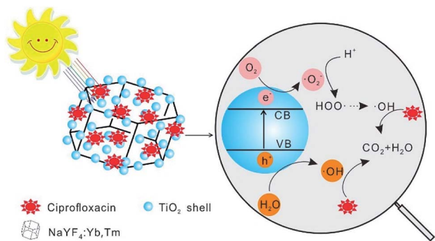
Scheme 1 Illustrated mechanism of photocatalytic degradation of CIP on \text{NaYF}_4:\text{Yb,Tm}@TiO_2 under Xe lamp irradiation.
