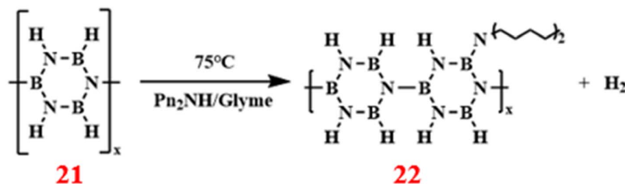
Scheme 16 Synthesis route of dipentylamine-modified polyborazine. 89
