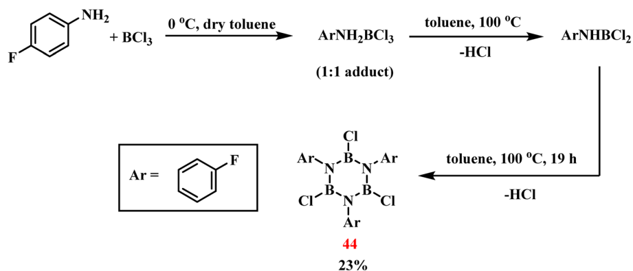
Scheme 31 Synthesis of 44 via pyrolysis of p -fluoroaniline with BCl 3 . 108
