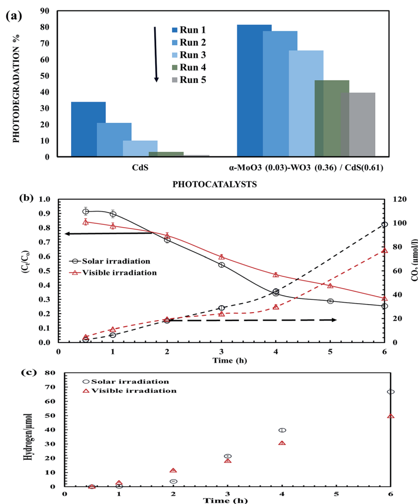
Fig. 6 (a) Photostability, (b) TOC photo-reduction, and (c) \text{H}_2 generation using \alpha\text{-MoO}_{3(0.03)}\text{-WO}_{3(0.36)}/\text{CdS}_{(0.61)} heterojunction photocatalyst under visible and solar lights.
