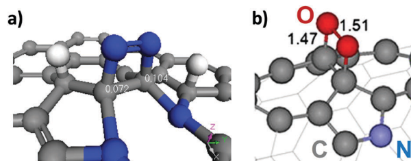
Fig. 24 (a) Model of N 2 activation at Stone–Wales defects with nearby N sites (in blue). (b) Model of O 2 activation at reactive C–C sites in Stone–Wales defects on the surfaces of graphene-like materials with specific curvature. Based on the model given in ref. 233 with permission from American Chemical Society, copyright 2014.
