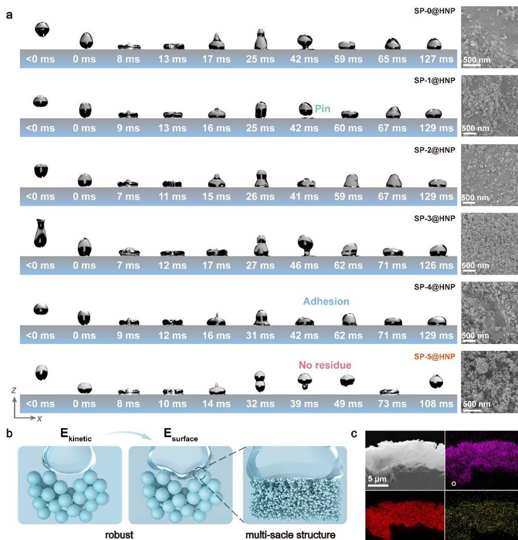
Fig. 3 Surface structures of SP-(0-5)@HNP and the non-equilibrium wetting behavior of low-velocity ( v \approx 0.64 m/s) water droplets on their surfaces. (a) High-speed camera images depicting the non-equilibrium wetting of low-velocity water droplets on the surfaces of SP-(0-5)@HNP and SEM images of their surface structures. (b) Schematic representation of the structure of SWDS. (c) Energy dispersive spectroscopy (EDS) characterization of SP-5@HNP.
