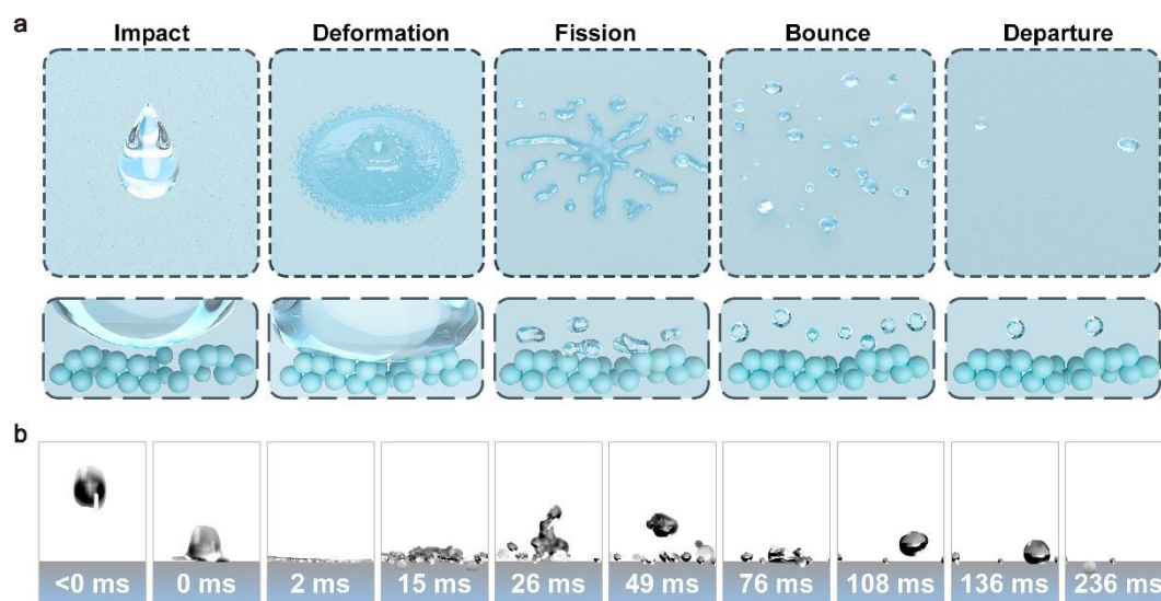
Fig. 5 Non-equilibrium wetting behavior of high-velocity ( v \approx 2.56 m/s) water droplets on the surface of SP-5@HNP. (a) Schematic illustration of the non-equilibrium wetting processes of high-velocity water droplets on the surface of SP-5@HNP. (b) High-speed camera images depicting the non-equilibrium wetting of high-velocity water droplets on the surface of SP-5@HNP.
