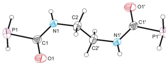
Fig. 3 Molecular structure of 2 . Thermal ellipsoids pictured at the 50% probability level. Symmetry operation \bar{1}: -x, -y, 1 - z . Selected bond distances ( \text{\AA} ) and angles (deg): P1–C1: 1.8633(12); C1–O1: 1.2275(15); C1–N1: 1.3256(15); N1–C2: 1.4549(15); C2–C2': 1.519(2); O1–C1–P1: 118.38(9); N1–C1–P1: 118.47(8); O1–C1–N1: 123.06(11).
