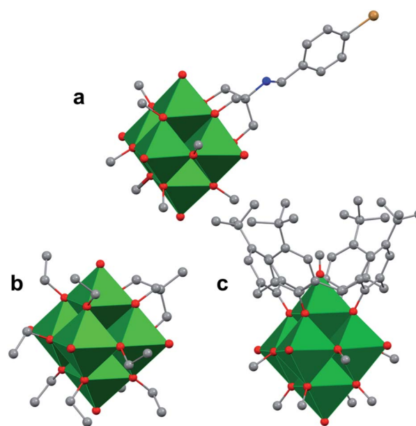
Fig. 11 Molecular structures of mixed-dentate POV-alkoxide clusters: (a) [V_6O_7(OCH_3)_9TRIS^{NC_7H_6Br}1^{-}] ; (b) [V_6O_7(OC_2H_5)_9(TRIS^{CH_3})1^{-}] ; and (c) [V_6O_6(OCH_3)_8(calix)1^{-}] . Colour code: V: green polyhedra, O: red, C: grey, N: blue, Br: orange. Hydrogen atoms, solvent molecules, and counter cations are removed for clarity.
