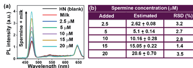
Fig. 6 (a) The upconversion luminescence spectra of pristine UCN@mSiO 2 @TDPM in water (HN, 100 mg/3 mL) and with varying amounts of spiked milk (spermine: 2.5–20 \mu\text{M} ). (b) Tabular representation of the relative standard deviation (RSD) of the estimated biogenic amine (spermine) in pre-treated milk employing the hybrid upconversion nanoprobe.
