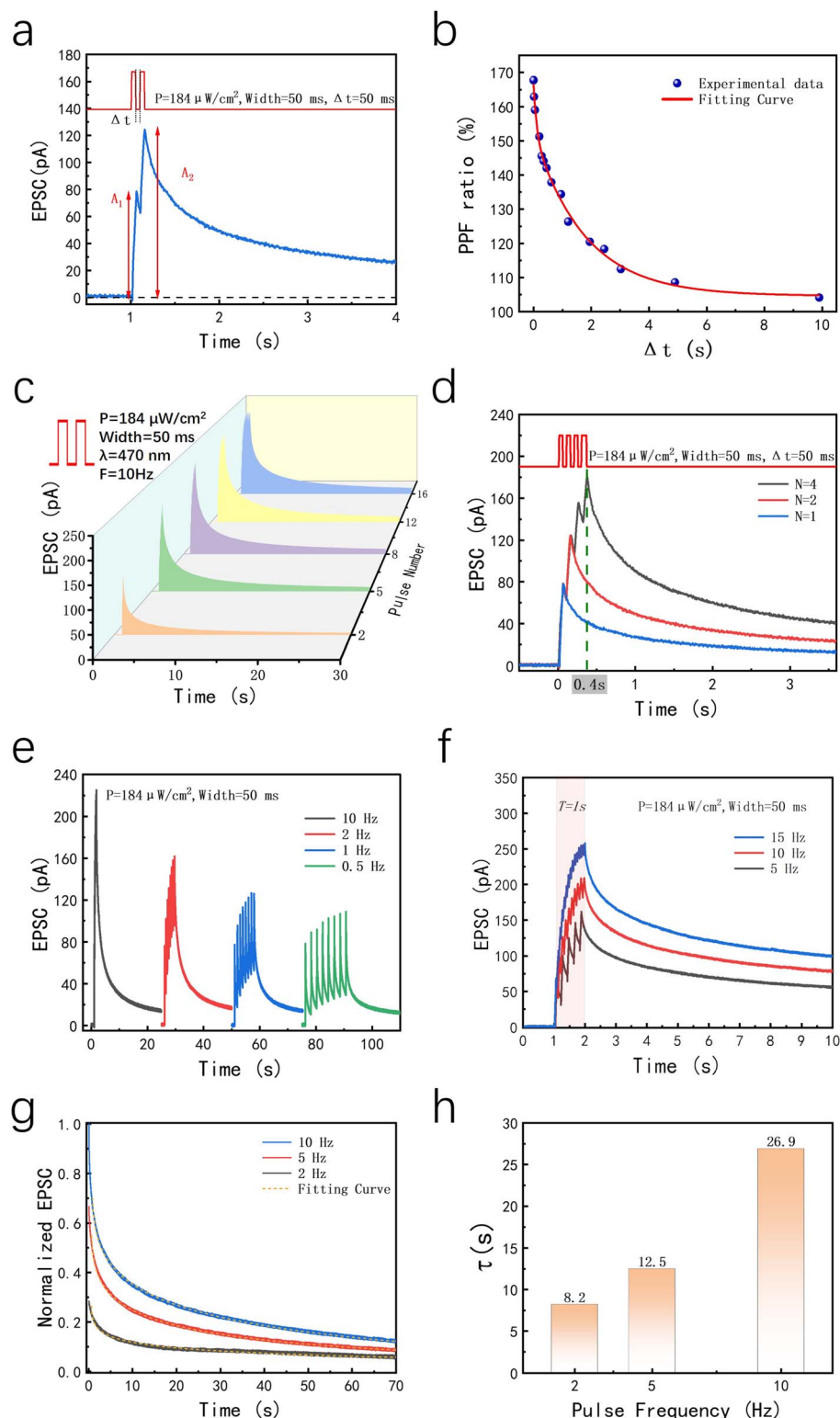
Fig. 3 Optoelectronic synaptic functions in Al/MoO 3 /CsFAMA/ITO synapses. (a) Photonic PPF stimulated by a pair of optical pulses ( P = 184 \mu\text{W}/\text{cm}^2 , width = 50 ms, \Delta t = 50 ms, \lambda = 470 nm). (b) PPF index (defined as A_2/A_1 ) depending on a series of time intervals ( \Delta t ). The EPSC stimulated by different (c) optical spikes, (d) numbers, (e) frequencies (10 spikes), and (f) a fixed time of T = 1 s. (g) and (h) Decay curves and time ( \tau ) depending on different frequencies in (f). All the read voltages applied above were 0 V.
