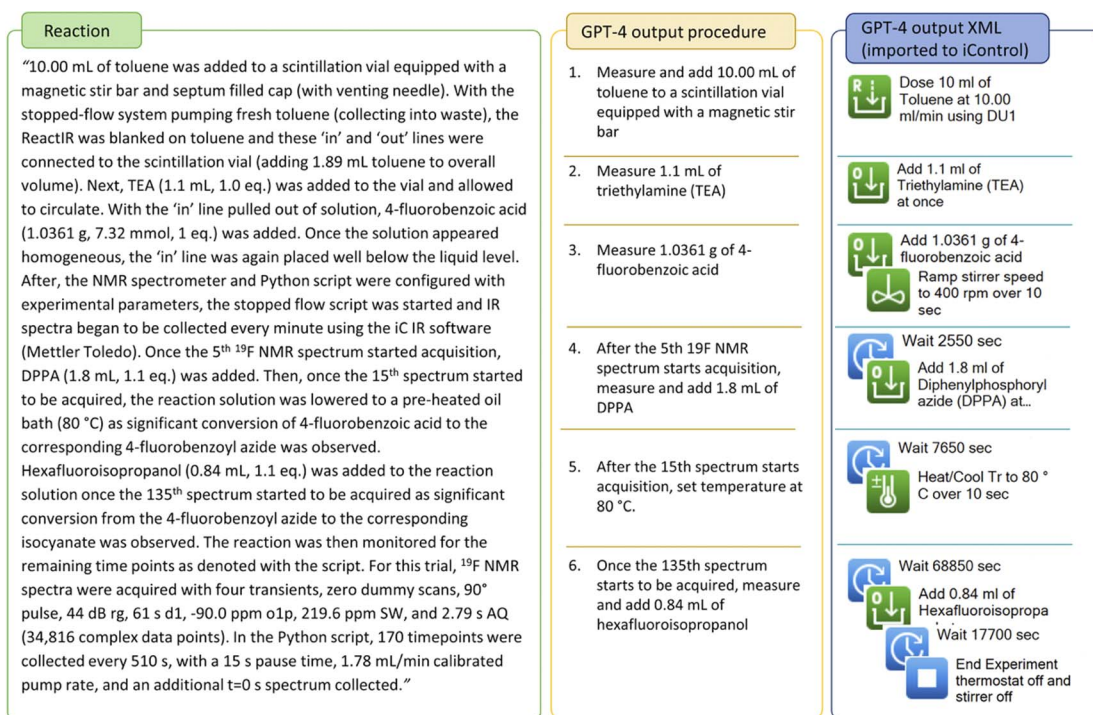
Fig. 7 Literature procedure of Curtius rearrangement, stepwise procedure and iControl operations generated by GPT-4.
