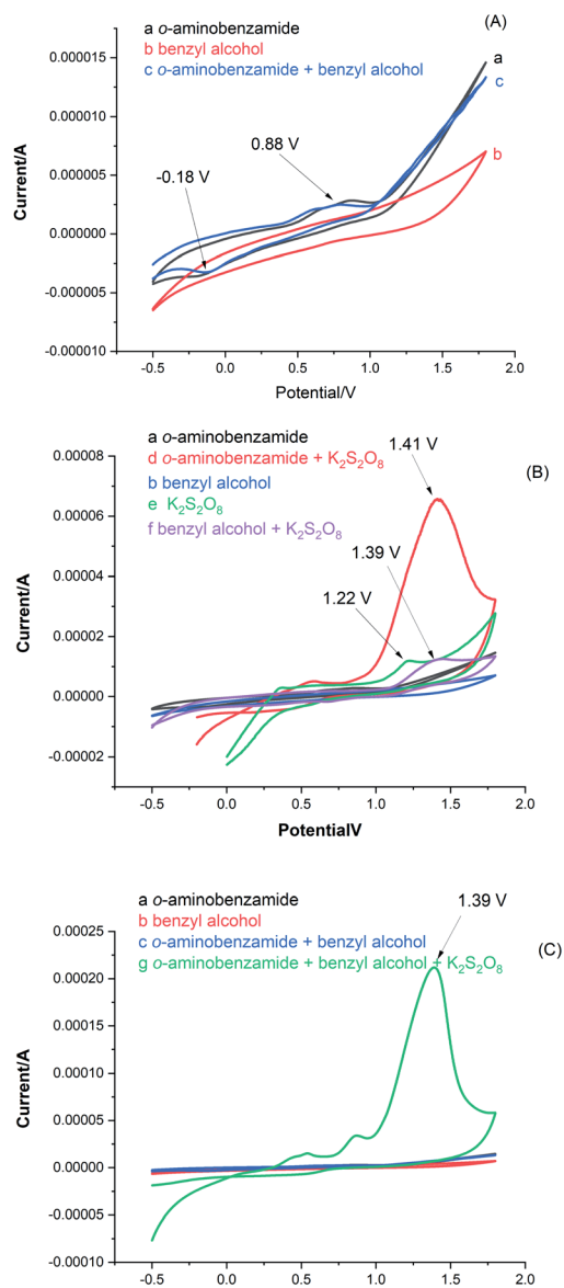
Fig. 2 Cyclic voltammograms of reactants and their mixtures in \text{CH}_3\text{CN}/\text{H}_2\text{O} on a glassy carbon working electrode (diameter: 3 mm) with a Pt wire and calomel electrode as the counter and reference electrode, respectively, at a scan rate of 0.1 \text{ V s}^{-1} . (A) (a) 1a , (b) 2a , (c) 1a + 2a ; (B) (a) 1a ; (d) 1a + \text{K}_2\text{S}_2\text{O}_8 ; (b) 2a ; (e) \text{K}_2\text{S}_2\text{O}_8 ; (f) 2a + \text{K}_2\text{S}_2\text{O}_8 ; (C) (a) 1a ; (b) 2a ; (c) 1a + 2a ; (g) 1a + 2a + \text{K}_2\text{S}_2\text{O}_8 .
