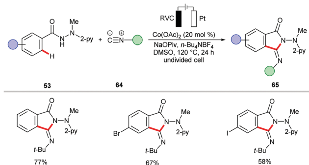
Scheme 19 Cobalt-mediated electrocatalytic C–H/N–H annulation with isocyanides 64 .
