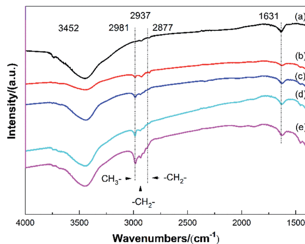
Fig. 6 FT-IR spectra of catalysts with different TOS. (a) 0 h; (b) 3 h; (c) 10 h; (d) 30 h; (e) 60 h.
