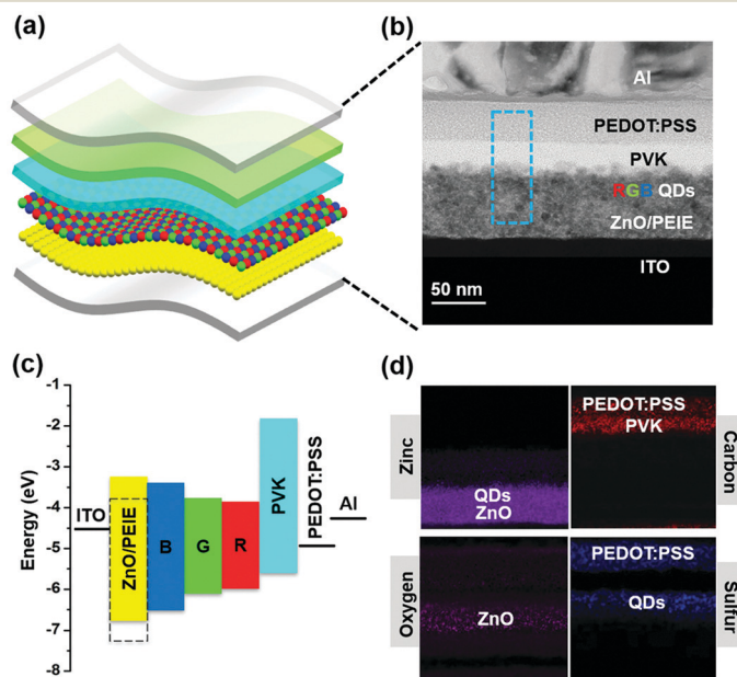
Fig. 1 (a) Device architecture and (b) cross-sectional TEM image of solution-processed, flexible white QLED. (c) Energy band diagram and (d) EDS compositional mapping images designated as a blue dotted rectangle in (b).
