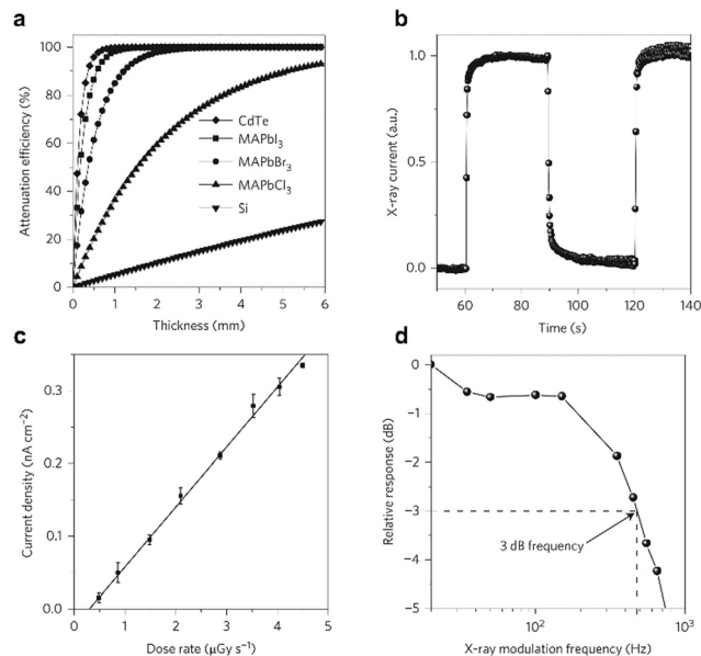
Fig. 11 (a) Attenuation efficiency of CdTe, MAPbI 3 , MAPbBr 3 , MAPbCl 3 and silicon to 50 keV X-ray photons versus thickness. (b) MAPPbBr 3 single-crystal device response to X-rays by turning the X-ray source on and off. (c) X-ray-generated photocurrent at various dose rates, down to the lowest detectable dose rate. (d) Normalized response as a function of input X-ray frequency showing that the 3 dB cutoff frequency is 480 Hz. Reproduced with permission. 60 Copyright 2016, Springer Nature.
