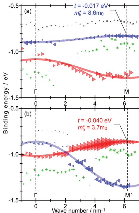
Fig. 22 The energy positions of the spectral components of ARUPS spectra taken in the (a) \Gamma - M and (b) \Gamma - M' directions plotted as a function of k_{\parallel} . The components attributed to the two valence bands are indicated as triangle marks, while those ascribed to some secondary factors are shown as \times , + , and * symbols. The size of each marks represents the intensity of the component. Reproduced from ref. 168 with permission (Copyright 2018, Materials Research Society).
