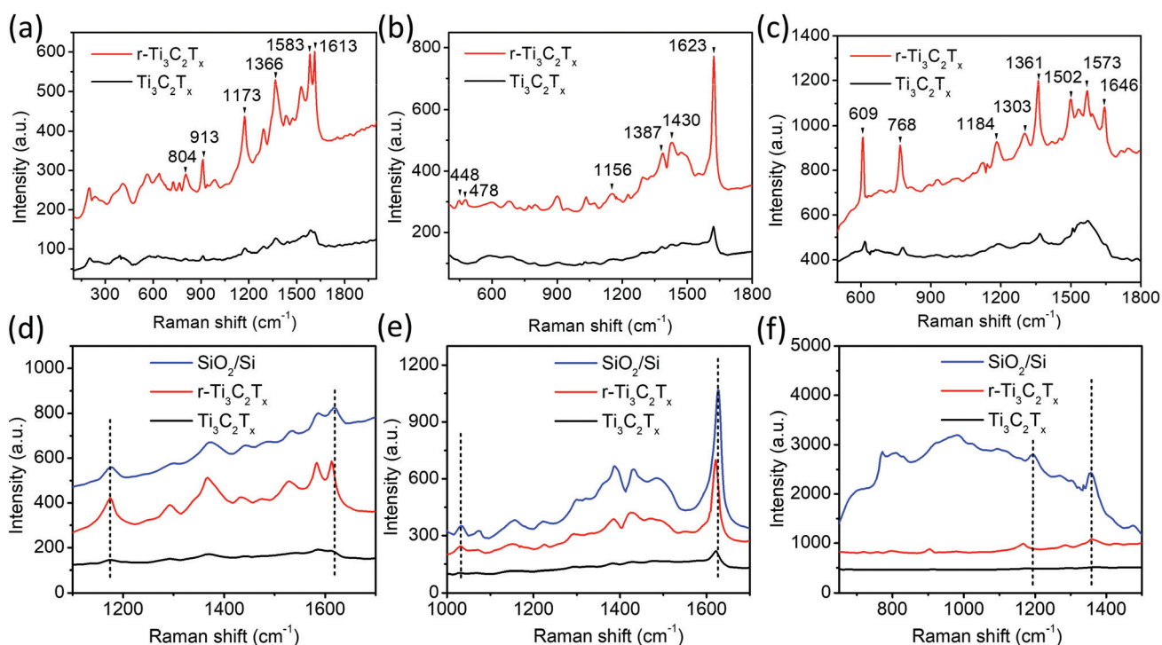
Fig. 6 SERS spectra of (a and d) CV, (b and e) MB, and (c and f) R6G collected on Ti_3C_2T_x/SiO_2/Si (black) and r-Ti_3C_2T_x/SiO_2/Si (red), and bare SiO_2/Si (blue) substrates. Concentration of dyes on SiO_2/Si substrate is 1 M in water.
