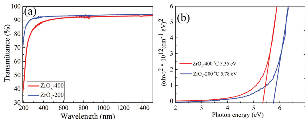
Fig. 4 (a) Total transmittance spectra of the ZrO_x dielectric film deposited at 200 °C and 400 °C and (b) corresponding bandgap extrapolation in the Tauc plots.
