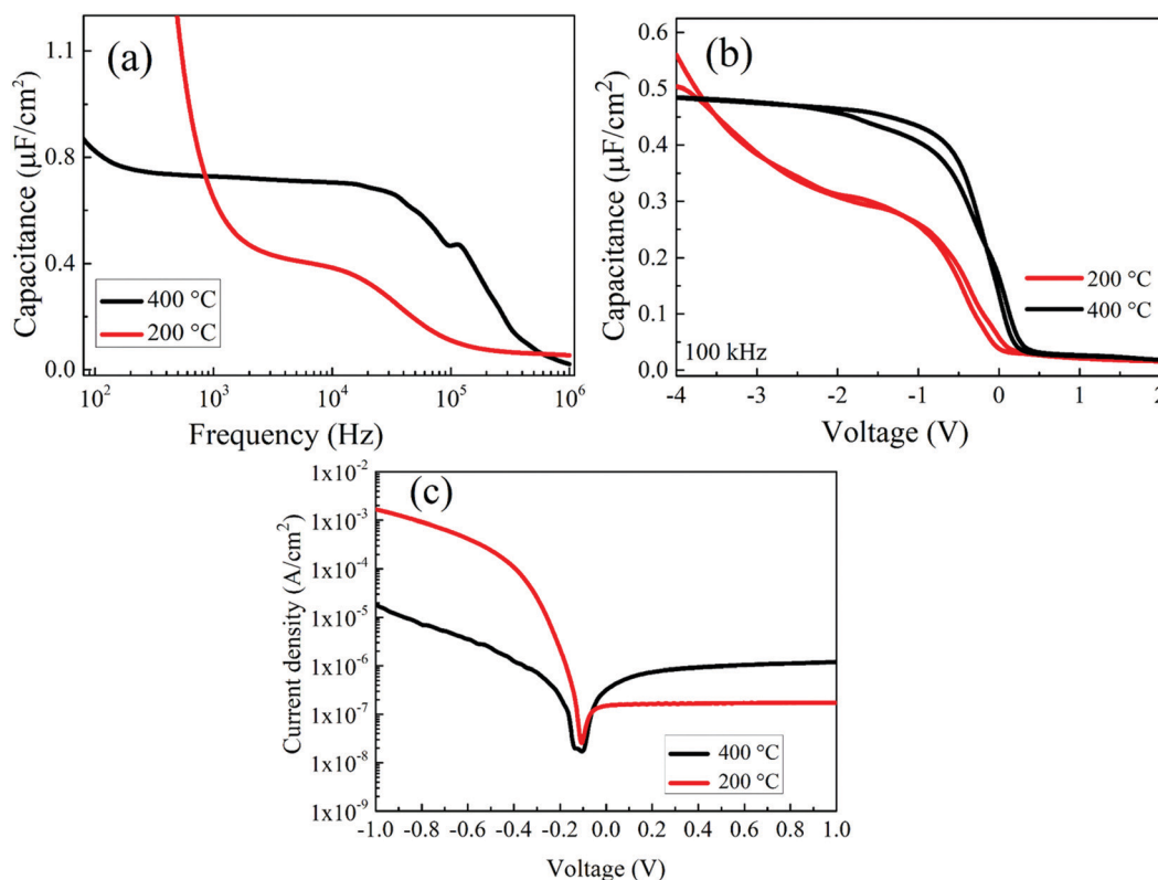
Fig. 5 (a) Capacitance–frequency curve, (b) capacitance–voltage, and (c) current–voltage characteristics of Al/p-type Si/ ZrO_x /Al MIS capacitors with the ZrO_x films obtained at various deposition temperatures.
