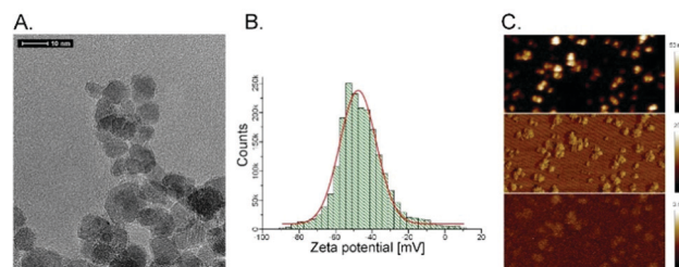
Fig. 1 SPIONs characterization: (A.) HR-TEM image, (B.) histogram of zeta potential values, (C.) AFM-MFM images, scan size = 1 \mu\text{m} (height – top, mechanical phase – middle and magnetic phase – bottom).
