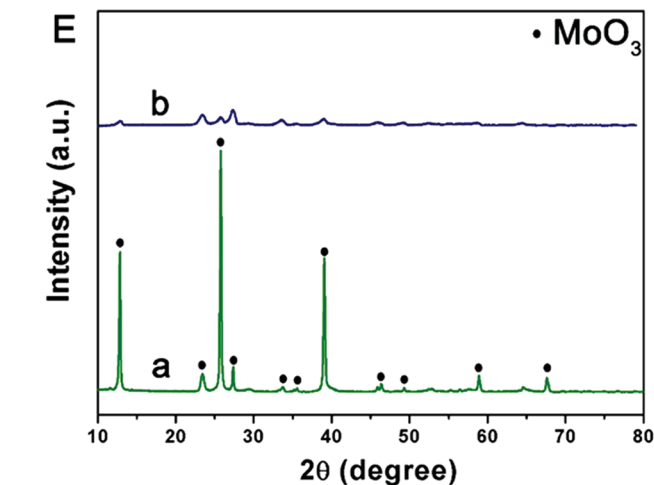
Fig. 1 SEM and TEM images of \text{MoO}_3 (A and B) and \text{MoO}_3 @PPy (C and D), and (E) XRD patterns of \text{MoO}_3 (a) and \text{MoO}_3 @PPy (b). Scale bars: 1 \mu\text{m} in (A–D).
