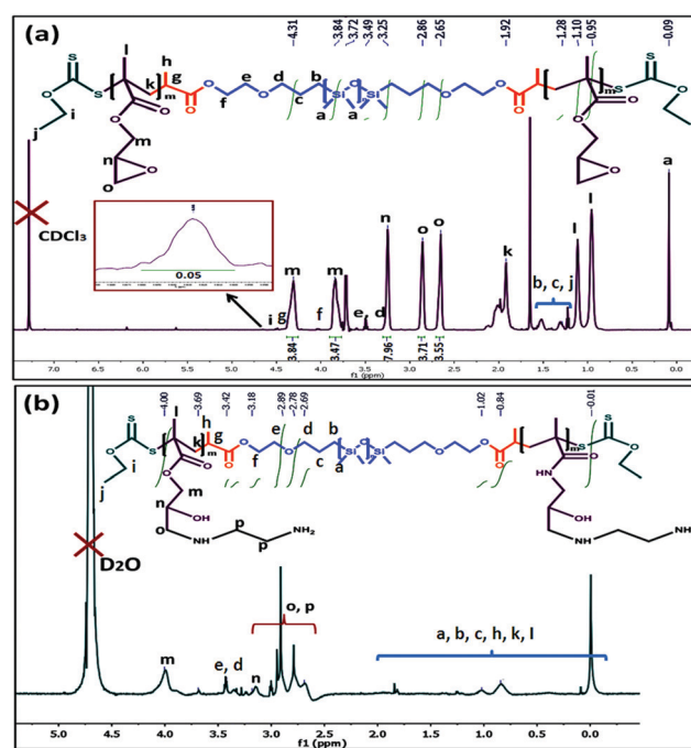
Fig. 2 ^1\text{H} NMR analysis of the (a) PGMA- b -PDMS- b -PGMA tri-block copolymer and (b) amine modified PDMS based tri-block copolymer (AmPGMA- b -PDMS- b -AmPGMA).
