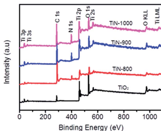
Fig. S3(a) XPS survey spectra of TiO 2 and TiN nanowires.
