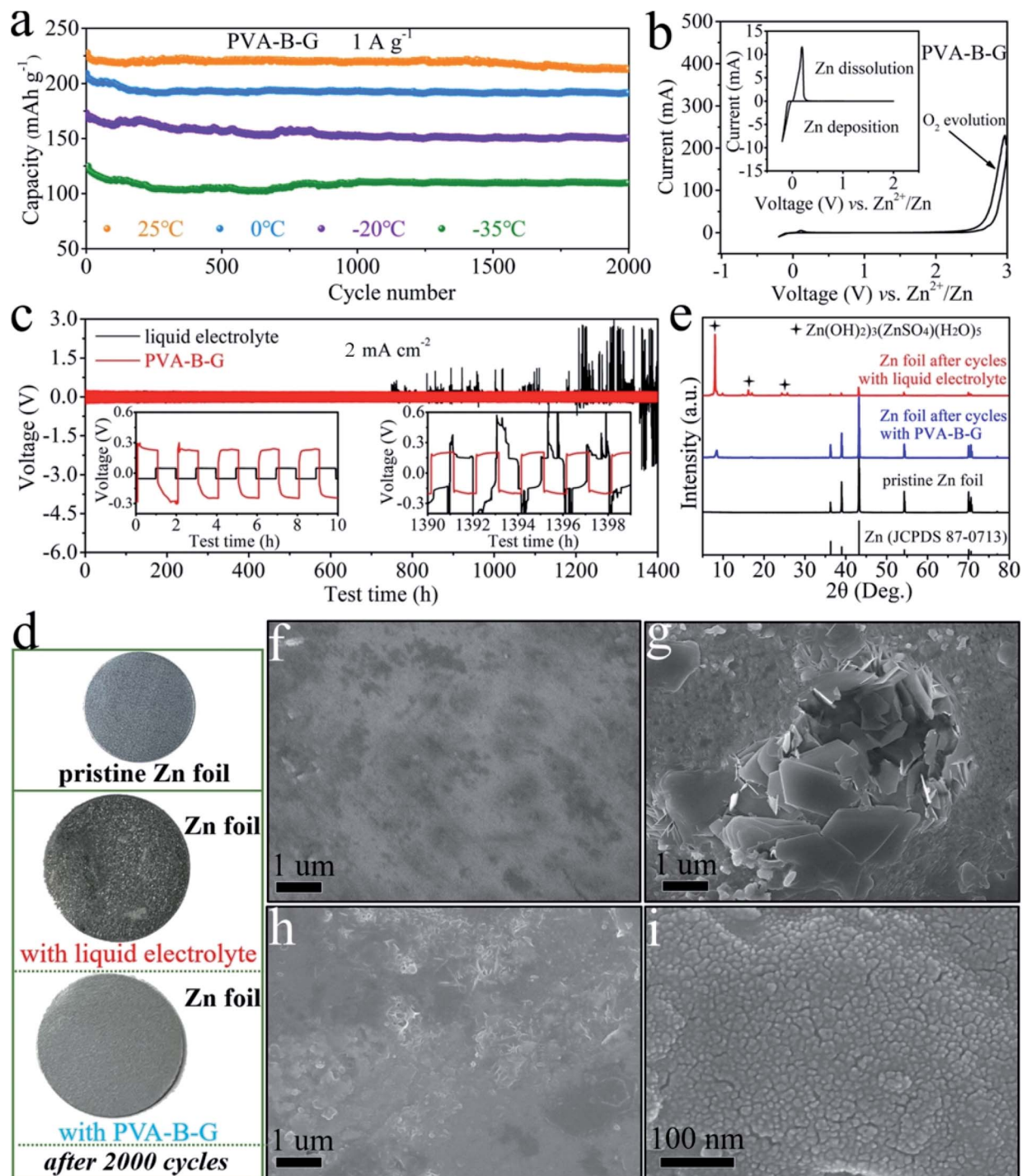
Fig. 5 (a) Cycling performances of the PVA-B-G battery at 1 A g -1 at different temperatures. (b) CV curve of Zn deposition/dissolution in a Zn//PVA-B-G//stainless steel cell between -0.2 and 3.0 V. (c) GCD curves of Zn//Zn symmetrical cells with PVA-B-G and liquid electrolytes cycled at 2 mA cm -2 (insets show the enlarged voltage profiles of the initial and last 10 h). (d) Photographs and (e) XRD patterns of the Zn foil at the pristine state and after 2000 cycles with different electrolytes. SEM images of (f) pristine Zn foil, (g) Zn foil with the liquid electrolyte after 2000 cycles, and (h and i) Zn foil with PVA-B-G after 2000 cycles.
