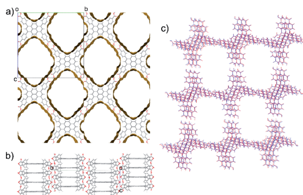
Fig. 3 Predicted porous structure of TBAP. (a) Viewed down the channels with the surface indicating the solvent accessible surface (probe radius 1.2 \text{ \AA} ) and (b) viewed perpendicular to the channels, showing the pyrene \pi -stacking. (c) An overlay of the predicted crystal structure 1 (red) and the experimental crystal structure TBAP- \alpha (blue).
