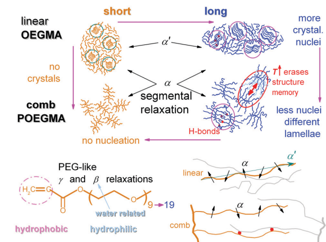
Scheme 3 Simplified model schemes for rationalizing the overall effects on crystallization (top) and describe the proposed origins of the segmental and local dynamics in the linear OEGMAs and comb-like POEGMAs (bottom).
