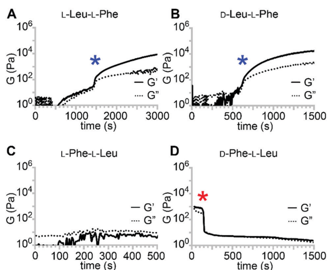
Fig. 1 Oscillatory rheology time sweeps for the four dipeptides at 40 mM. Blue stars mark sol-to-gel transitions for the two gelators L -Leu- L -Phe and D -Leu- L -Phe; the red star in (D) marks gel-to-sol transition for the metastable gel formed by D -Phe- L -Leu.
