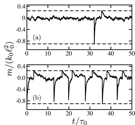
Fig. 3 Time dependence of dimensionless force dipoles \tilde{m} = m/(k_0\ell_0^2) on time for (a) \tilde{v}_0 = 0.03 and (b) \tilde{v}_0 = 3 . Dashed lines show the lower bound \tilde{m}_{\min} = -0.9 for the deterministic oscillatory dimer and the absolute upper bound \tilde{m}_{\max} = 0.25 for force dipoles.
