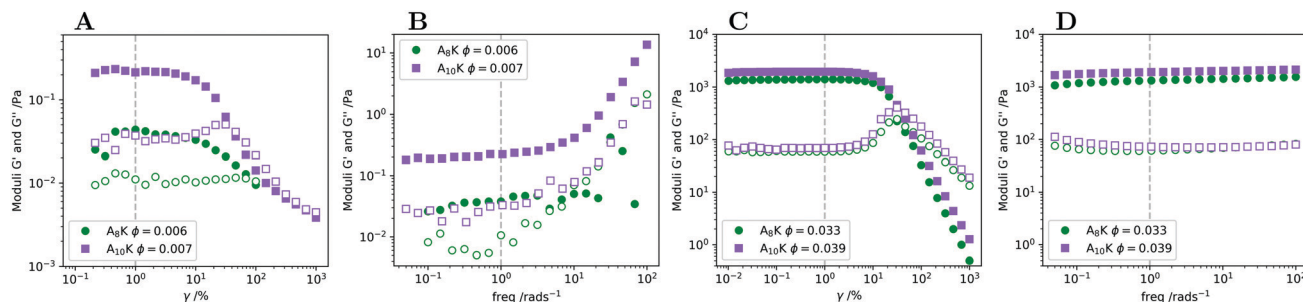
Fig. 5 Amplitude and frequency sweeps for the two regions above \phi \approx 0.005 with concentrations \phi \approx 0.006 in (A) and (B), and \phi \approx 0.033 in (C) and (D). G' is shown as filled symbols and G'' are hollow. (A) and (C) Show amplitude sweeps with similar behavior, G' > G'' at low deformations and a cross-over to a G' < G'' regime at higher deformations. (B) and (D) Show frequency sweeps of the lower and higher concentrations respectively. Dashed vertical lines point out the strain and frequency values used for the respective strain and frequency sweeps. Noisy data at low frequencies and strains is attributed to measurements close to the detection limit of the instrument.
